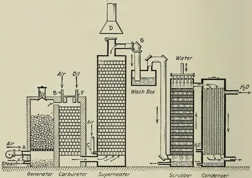
FIG. 101.—Lowe Water-gas Plant.
